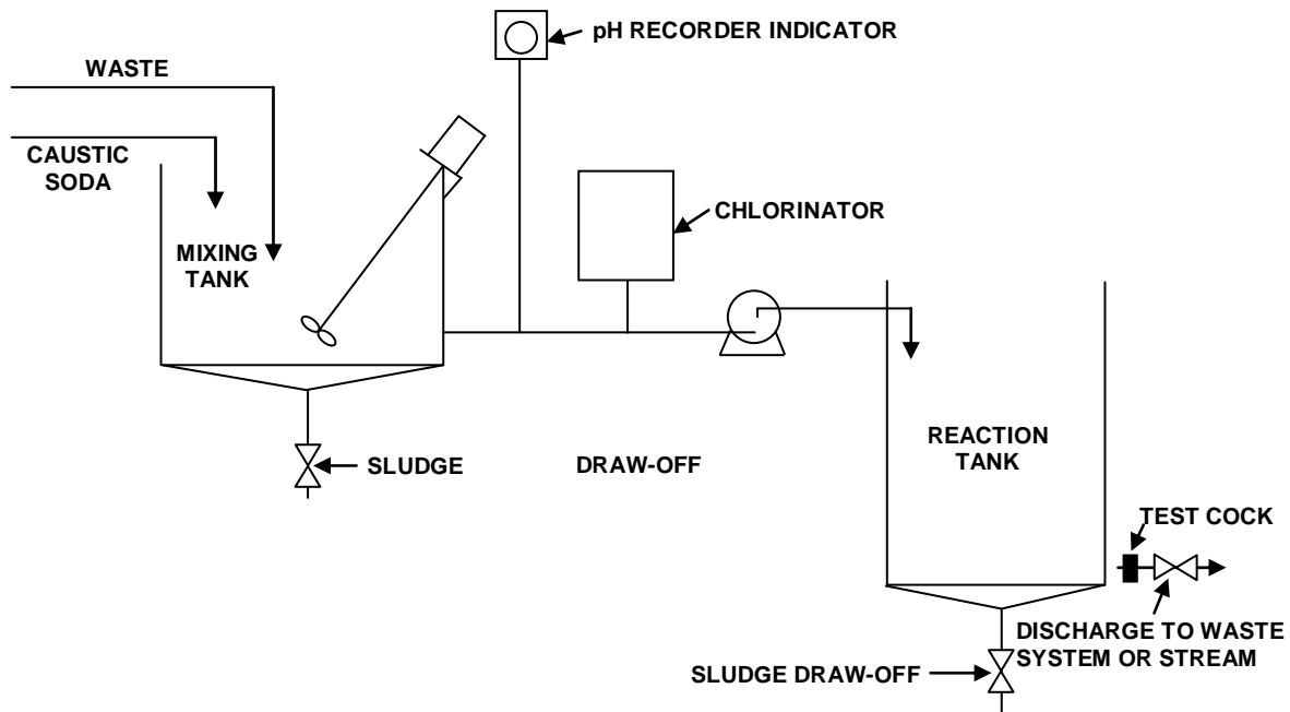
Figure 10 - 4. Cyanide treatment
